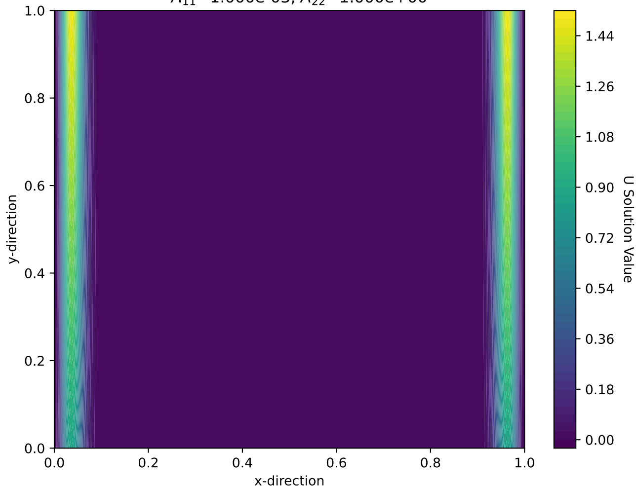
RBF-FD Approximate Solution (Contour): A_{11}=1.000\text{e-}03 , A_{22}=1.000\text{e+}00
